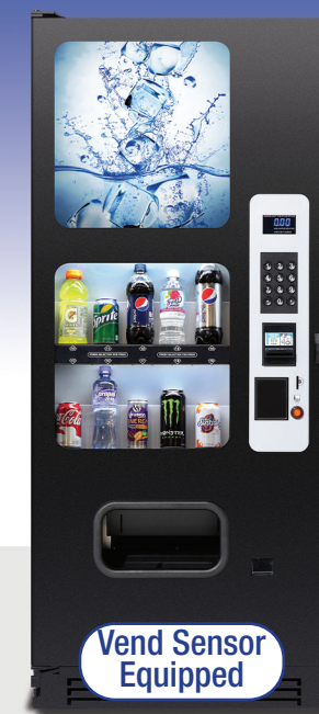
AB10/50 Bottle & Can Vendor 72" x 31.75"W x 36.5"D *Ship Weight 671 lbs, 10 selections Capacity: 500-12oz cans / 240-20 oz bottles or combination of cans and bottles Standard vend sizes in ounces: 12, 16.9, 20 & 24 (Optional kit needed for 250ml Energy Drink cans) Card reader available
